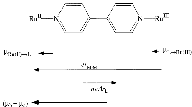
Fig. 3. Illustration of the contributions to the diabatic dipole-moment change in the MMCT transition in [(\text{NH}_3)_5\text{Ru}^{\text{II}}-4,4'\text{-bpy}-\text{Ru}^{\text{III}}(\text{NH}_3)_5]^{5+} . er_{\text{M-M}} is the primitive dipole-moment change due to the transfer of an electron between the Ru centers, ne\Delta r_{\text{L}} is the dipole-moment reduction due to the polarization of the electrons of the bridging ligand, \mu_{\text{Ru(II)}\rightarrow\text{L}} and \mu_{\text{L}\rightarrow\text{Ru(III)}} are dipoles resulting from metal-to-ligand and ligand-to-metal electron delocalization, respectively, and (\mu_{\text{b}} - \mu_{\text{a}}) is the diabatic dipole-moment change for the MMCT transition.
